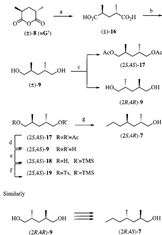
Scheme 5. Synthesis of the building blocks (2 S ,4 R )- and (2 R ,4 S )- 7 : reagents: (a) H 2 O, heat; then recrystallization from CHCl 3 (20%); (b) BH 3 ·SMe 2 , THF (80%); (c) CH 2 =CHOAc, lipase AK (twice) [26% of (2 S ,4 S )- 17 ; 26% of (2 R ,4 R )- 9 ]; (d) K 2 CO 3 , MeOH (99%); (e) n BuLi, TMSCl, THF (88%); (f) TsCl, Et 3 N, CHCl 3 (quant.); (g) (1) EtMgBr, Li 2 CuCl 4 , THF, (2) dil. HCl (87%)
