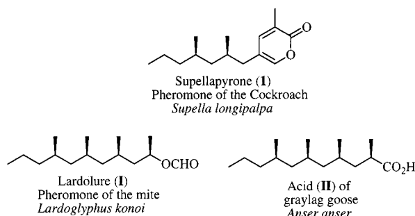
Scheme 1. Structures of supellapyrone ( 1 ) and related compounds
