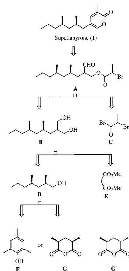
Scheme 2. Retrosynthetic analysis of supellapyrone (1)
