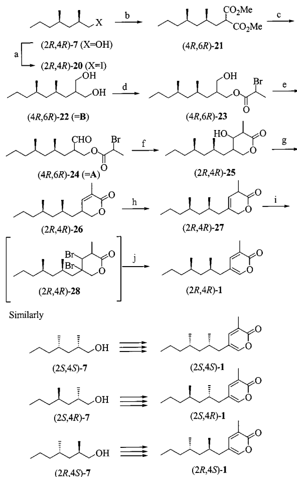
Scheme 6. Synthesis of supellapyrone (2 R ,4 R )- 1 and its stereoisomers: reagents: (a) I 2 , Ph 3 P, imidazole, DMF (99%); (b) CH 2 (CO 2 Me) 2 , NaH, THF (76%); (c) NaBH 4 , THF/MeOH (85%); (d) n BuLi, MeCHBrCOBr, THF (78%); (e) CrO 3 ·HCl·C 5 H 5 N (PCC), MS 4 Å, CHCl 3 ; (f) SmI 2 , THF [71% based on (4 R ,6 R )- 23 ]; (g) MsCl, DMAP, CHCl 3 (63%); (h) KN(SiMe 3 ) 2 , THF/HMPA; then dil. HCl (74%); (i) Br 2
