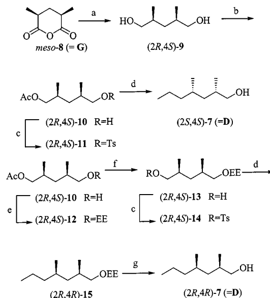
Scheme 4. Alternative synthesis of the building blocks (2 R ,4 R )- and (2 S ,4 S )- 7 : reagents: (a) LiAlH 4 , THF (80%); (b) CH 2 =CHOAc, lipase AK, THF (72%); (c) TsCl, C 5 H 5 N (quant.); (d) EtMgBr, Li 2 CuCl 4 , THF [87% for (2 S ,4 S )- 7 ; 77% for (2 R ,4 R )- 15 ]; (e) CH 2 =CHOEt, TsOH (96%); (f) K 2 CO 3 , MeOH (98%); (g) TsOH, MeOH (78%)
